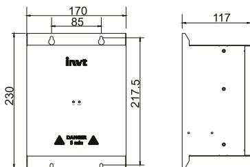
Installation dimension
